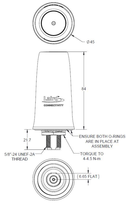
Figure 2: FTRA6971M5Px mechanical drawing
