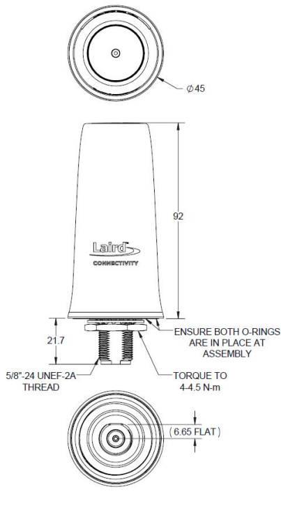
Figure 1: FTRA6171M5Px mechanical drawing
