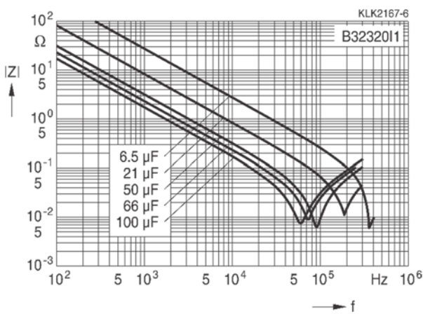
Impedance Z versus frequency f (Typical values)
