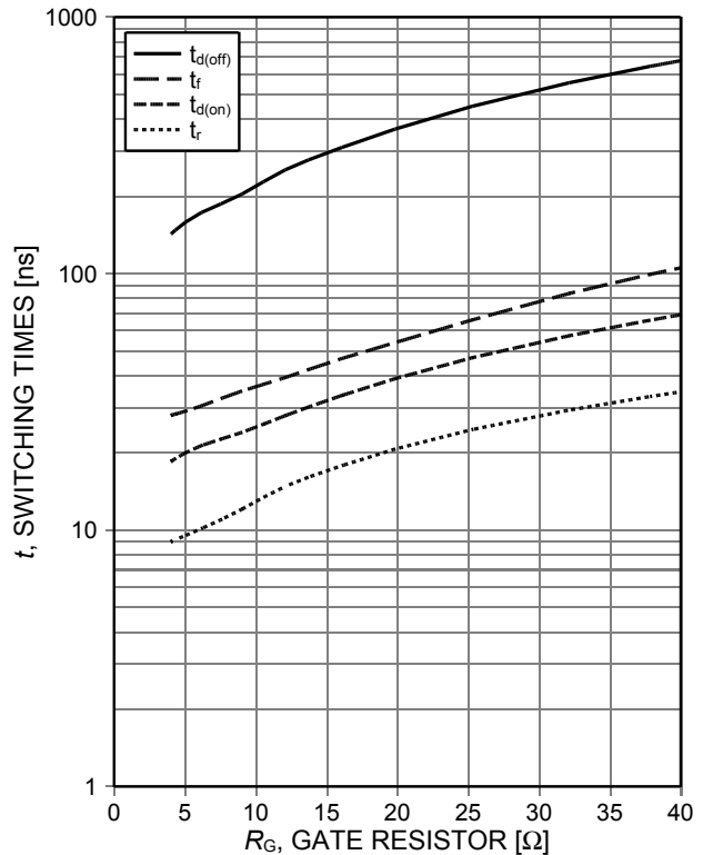
Figure 8. Typical switching times as a function of gate resistor (inductive load, T_{vj}=150^\circ\text{C} , V_{CE}=400\text{V} , V_{GE}=15/0\text{V} , I_c=37.5\text{A} , Dynamic test circuit in Figure E)
