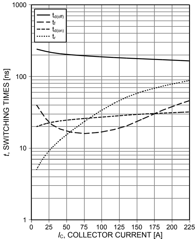
Figure 7. Typical switching times as a function of collector current (inductive load, T_{vj}=150^\circ\text{C} , V_{CE}=400\text{V} , V_{GE}=15/0\text{V} , R_G=9\Omega , Dynamic test circuit in Figure E)
